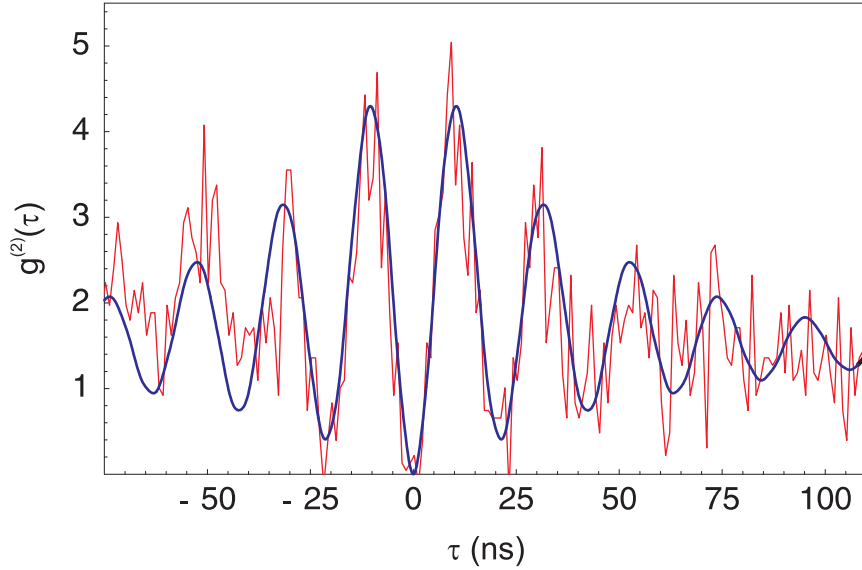
Figure 3.12.: Measured (red curve) and calculated (blue curve) second order correlation function. The theoretical correlation function was numerically calculated for a four level system with our experimental laser parameters [68]. For comparison, the measured data was background correct using the known dark count and signal rates of the photo detectors.
