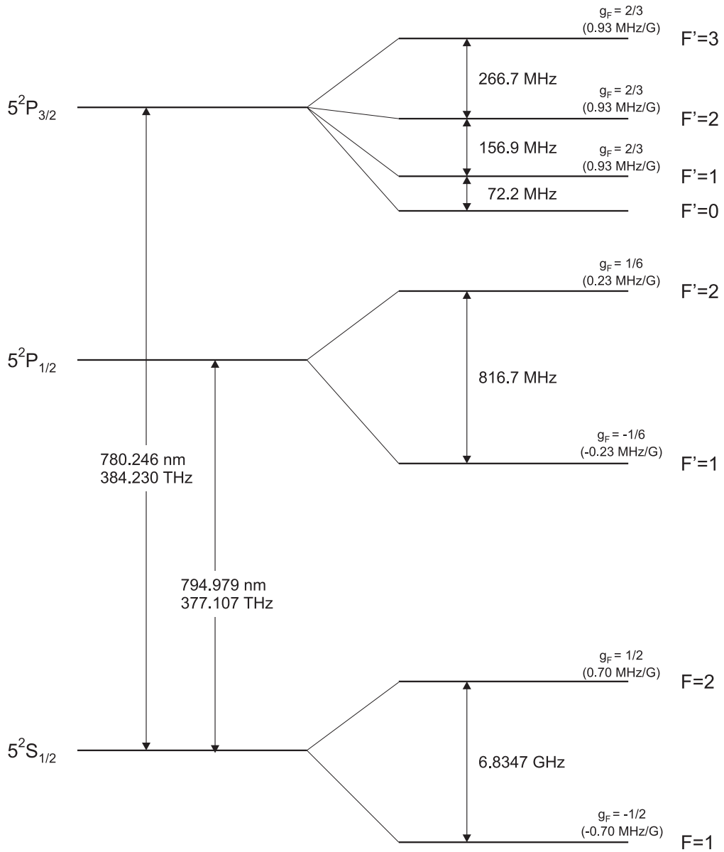
Figure A.3.: Hyperfine structure of the D_1 and D_2 transitions of ^{87}\text{Rb} [75].
