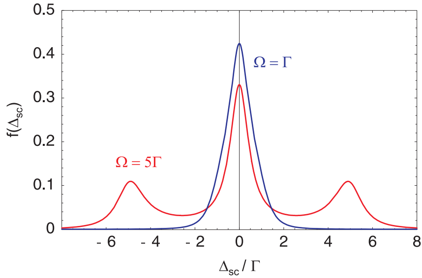
Figure 3.14.: Incoherent part of the fluorescence spectrum for resonant scattering ( \Delta = 0 ) for two different Rabi frequencies \Omega = \Gamma and \Omega = 5\Gamma . At low excitation power the spectrum consists only of a single peak centered at the laser wavelength. For stronger driving fields two side bands appear at the positions \omega \pm \Omega .
