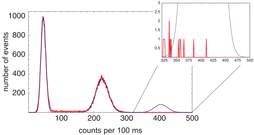
Figure 3.7.: Histogram of the fluorescence counts per 100 ms from a total measurement time of more than five hours. The red data corresponds to the measured number of occurrences of the respective count rate. The blue curve is a theoretical fit to the first two peaks assuming Poissonian occupation statistics of the dipole trap. The fluorescence events in the first peak are caused by the background count rate of the detector and the second and third peak correspond to the cases with one or two atoms inside the dipole trap. The inset shows a magnification of the region around the third peak. The probability to see two (or more) atoms inside the dipole trap is nearly zero and therefore clearly differs from a Poissonian distribution expected for non-interacting atoms.
