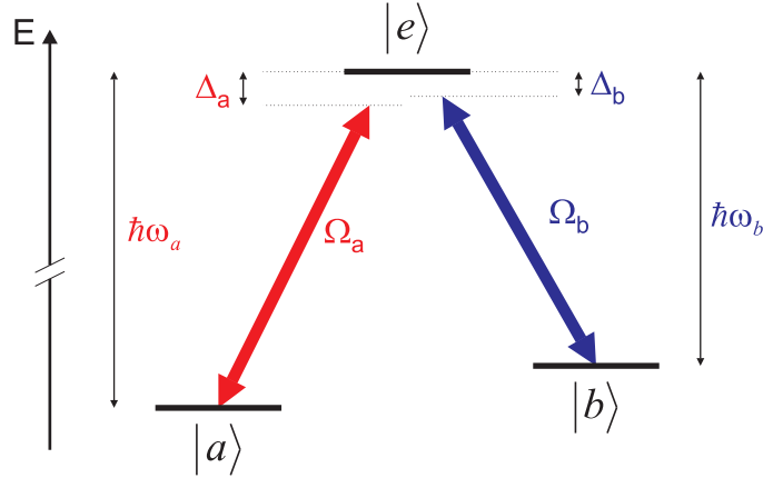
Figure 4.5.: Atomic system consisting of two stable ground states |a\rangle and |b\rangle and an excited state |e\rangle . Two light fields \Omega_a and \Omega_b – nearly resonant to the transitions |a\rangle \rightarrow |e\rangle with frequency \omega_a and |b\rangle \rightarrow |e\rangle with frequency \omega_b – are incident on the atom.
