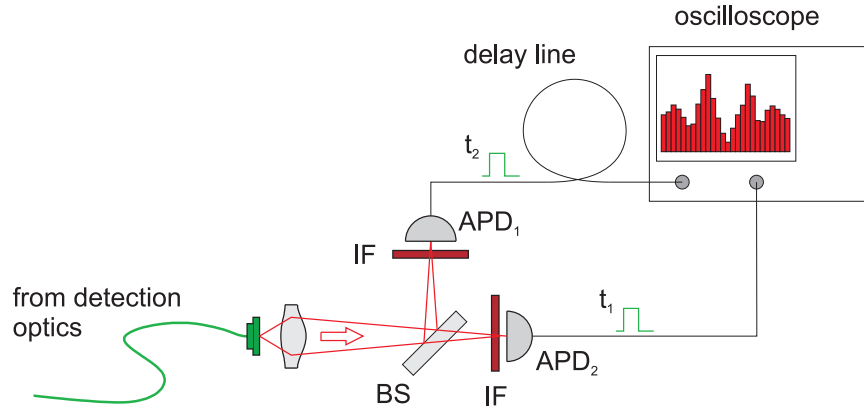
Figure 3.10.: Hanbury-Brown Twiss setup [79] for the measurement of the second order correlation function of the atomic fluorescence light. A 50/50 beamsplitter sends the incoming fluorescence onto two avalanche photo diodes. A storage oscilloscope histograms the differences of detection times \tau = t_1 - t_2 of photon pair events. Due to electrical reasons one of the two detection signals is delayed using a 70 ns delay line.
